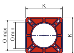
Burner flange
