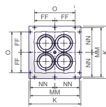
100 mm Burner flange
