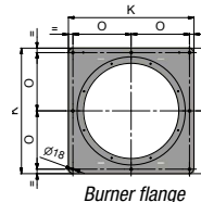
Burner flange
