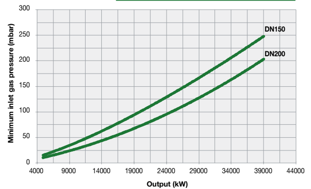
HTP3000 PR-MD with pneumatic valves
