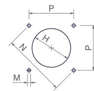
Suggested boiler drilling
