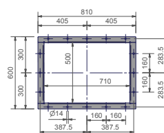
Air inlet flange
