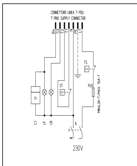
Fig. 22 - Conector 7-polos
