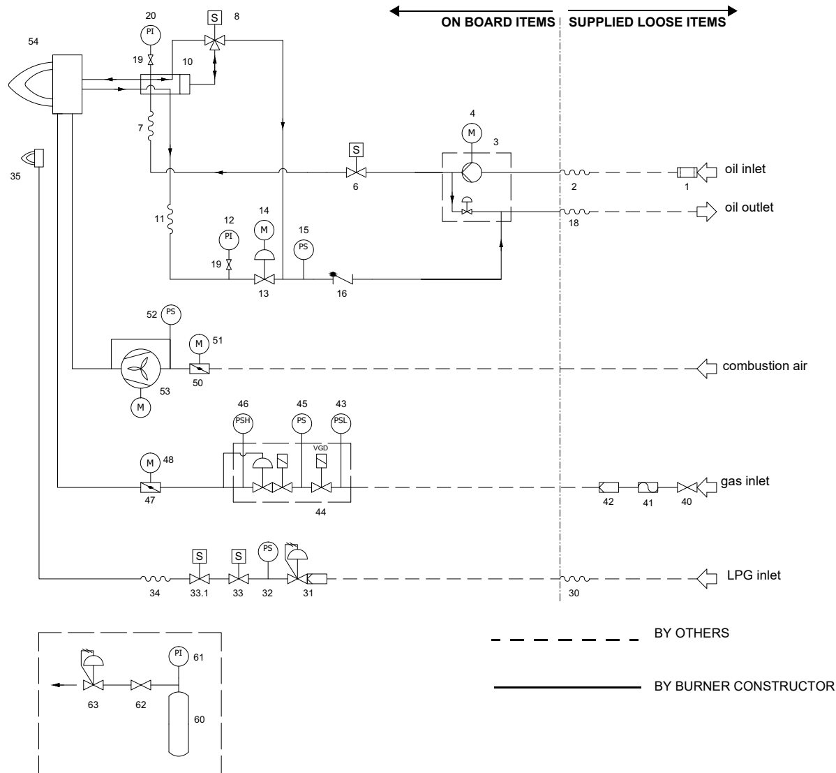
Fig. 1 - 3I2MG-20 v0 Hydraulic diagram - nozzle G, KV
