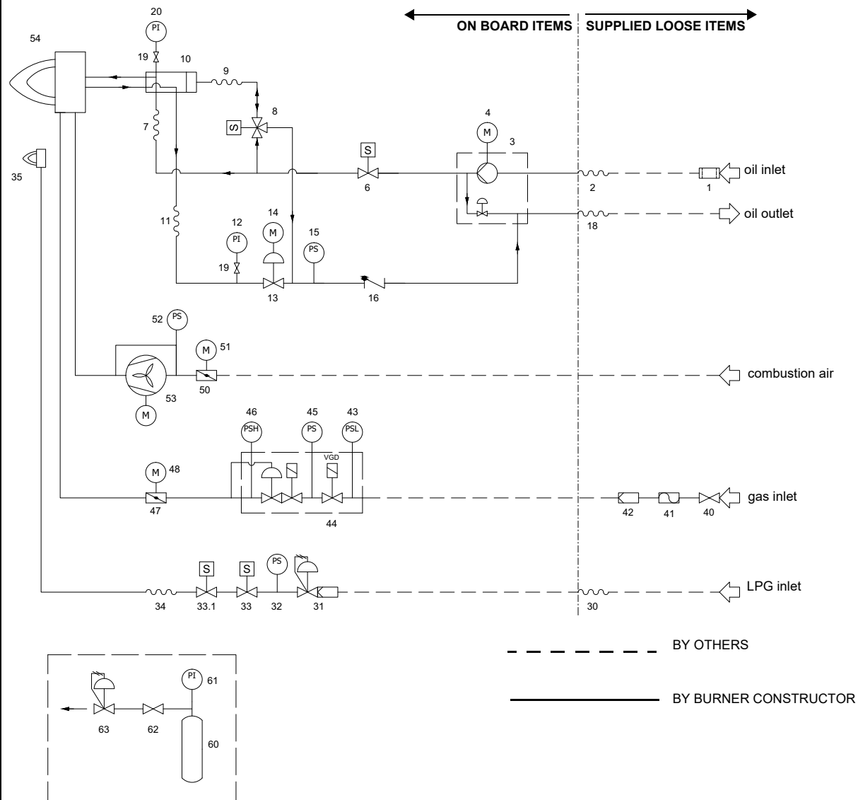
Fig. 1 - 3I2MG-19 v0 Hydraulic diagram - nozzle M3
