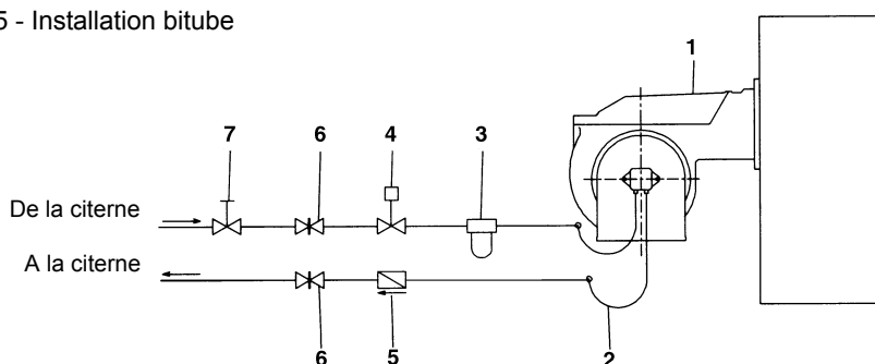
Fig. 5 - Installation bitube
