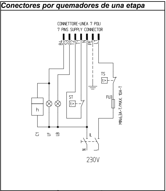
Conector 7-polos
