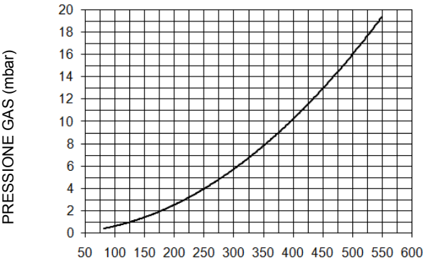
KRBY515 VS
