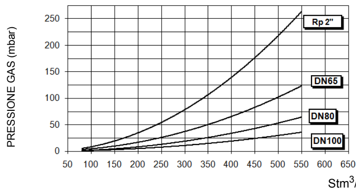
KRBY515 VS
