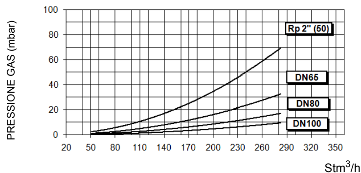
KRBY93 VS
