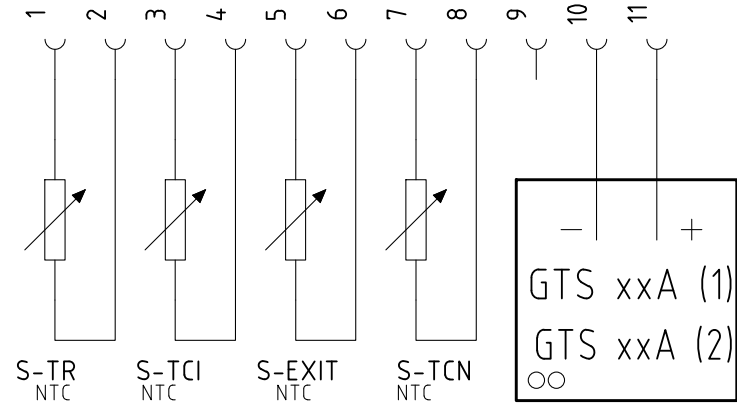
QGG - PROBE_F CONNETTORE SONDE [MCX06C] [MCX06C] PROBE CONNECTOR
