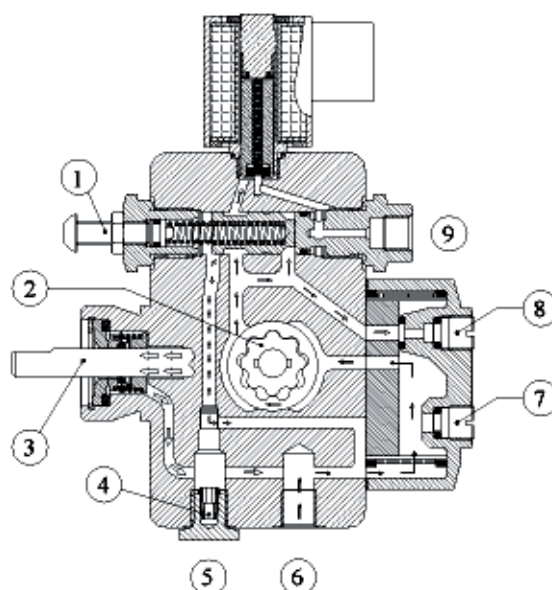
INSTALLATION MONOTUBE
