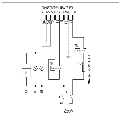
Fig. 8 - Conector 7-polos
